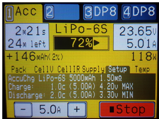
Figure 4 - Charger Setup
